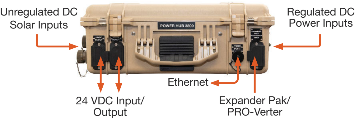
Figure 5. Overview of Power Hub connections
